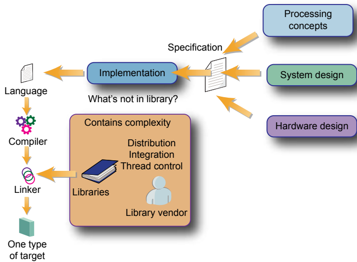
Figure 2: Gedae development
